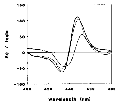
FIGURE 2 Soret region TRMCD spectra at 100–220 ns (----) and 10–12 \mu\text{s} (.....) after photolysis of 8 \mu\text{M} CcO-CO. Shown for comparison are the equilibrium MCD of CcO-CO (—) and reduced CcO (—). MCD is calculated from Eqs. 2 and 4. Magnetic field strength is 0.64 T.
